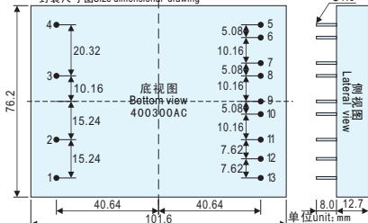
封装尺寸图Size dimensional drawing
