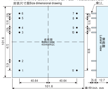
封装尺寸图Size dimensional drawing
