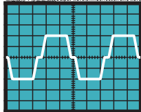
输出波形:修正正弦波Output waveform:Correction sine wave
